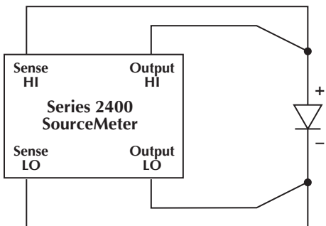
Figure 5. Four-wire connection
