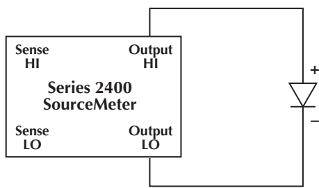
Figure 4. Two-wire connection
